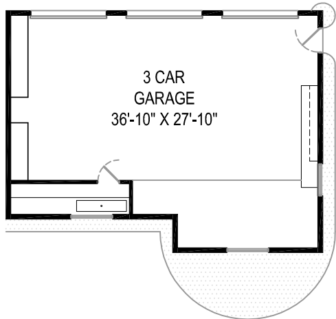
GARAGE PLAN
